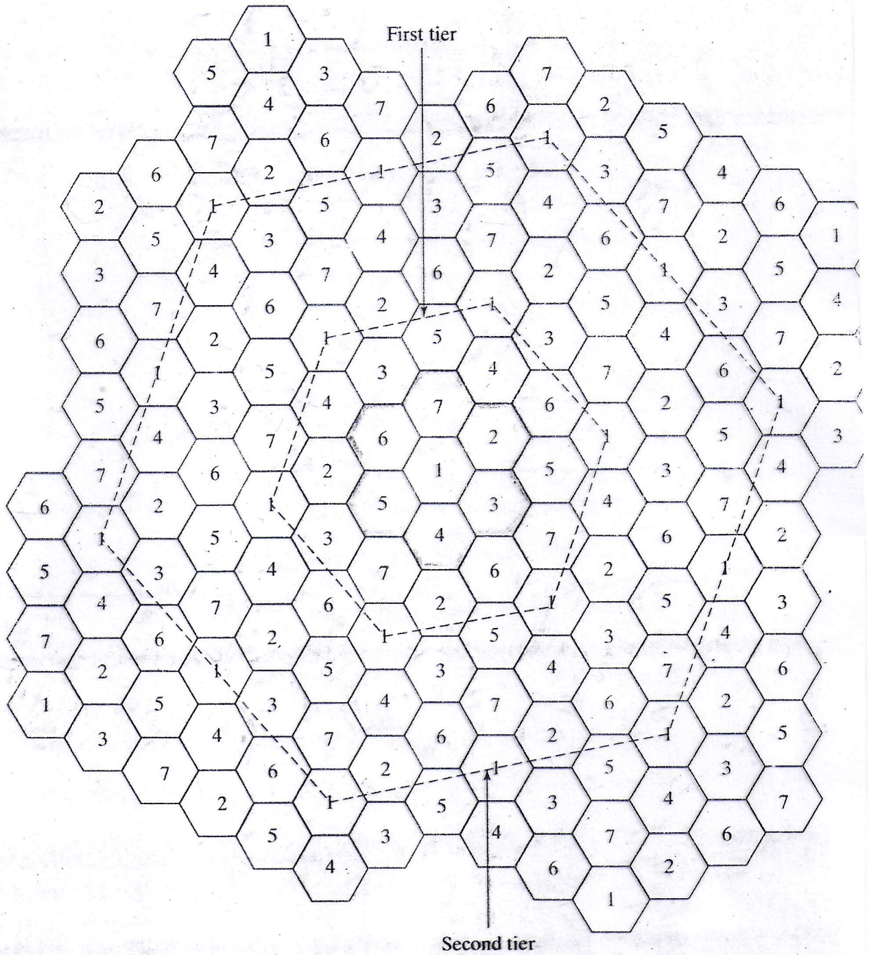
Figure 5.4 Two tiered interfering cells with N = 7 .
